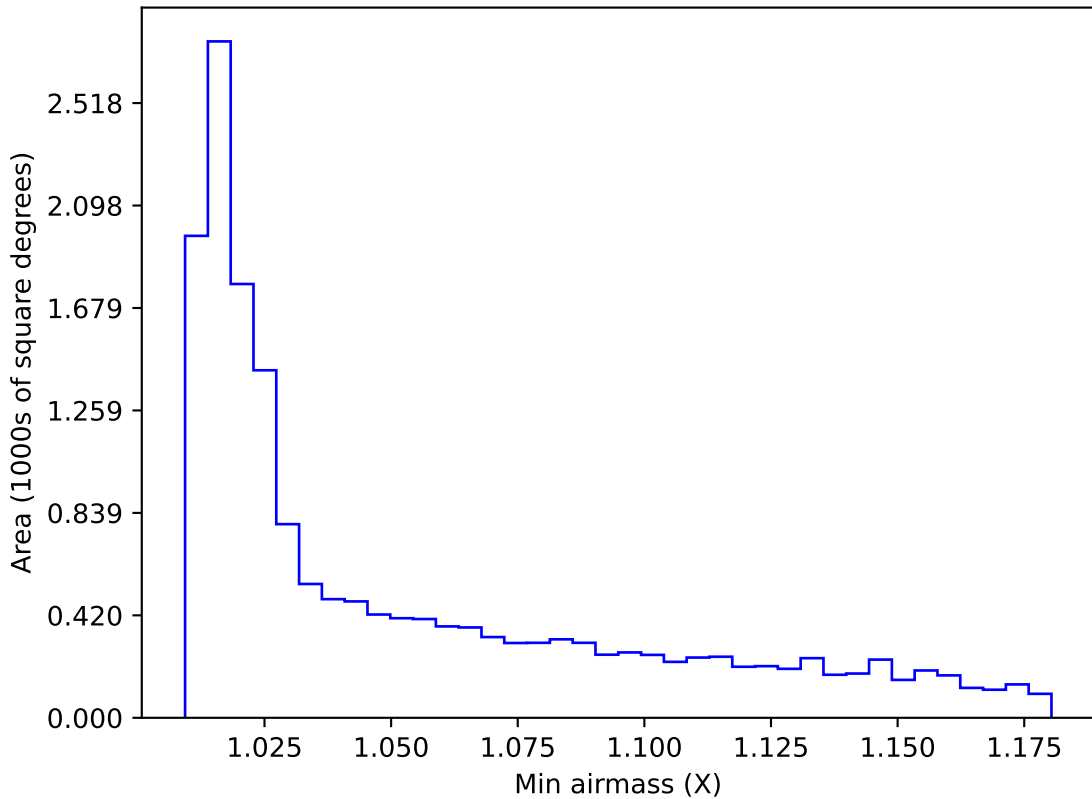
retro_baseline_v2.0_10yrs WFD i band: Min airmass
