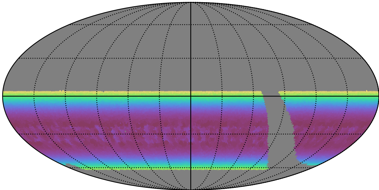
retro_baseline_v2.0_10yrs WFD g band: Min airmass
