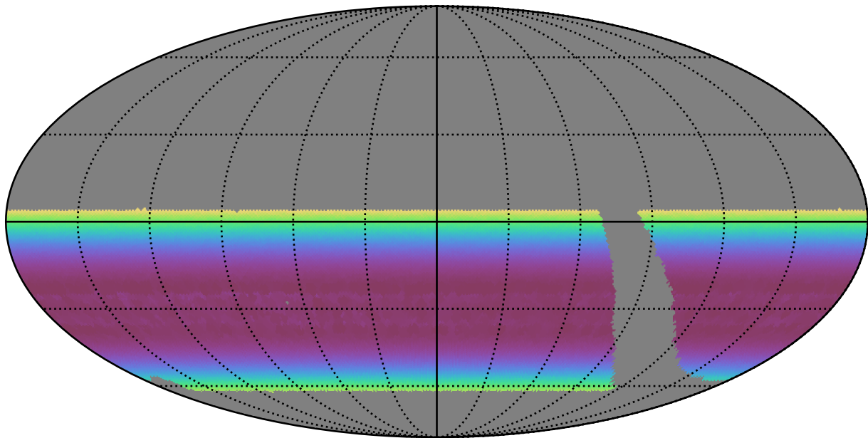
retro_baseline_v2.0_10yrs WFD all bands: Min airmass
