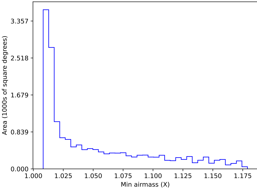
retro_baseline_v2.0_10yrs WFD all bands: Min airmass
