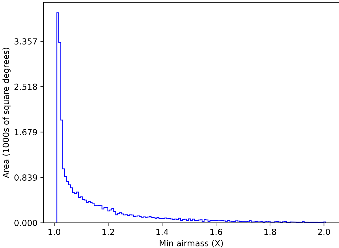
retro_baseline_v2.0_10yrs All sky z band: Min airmass
