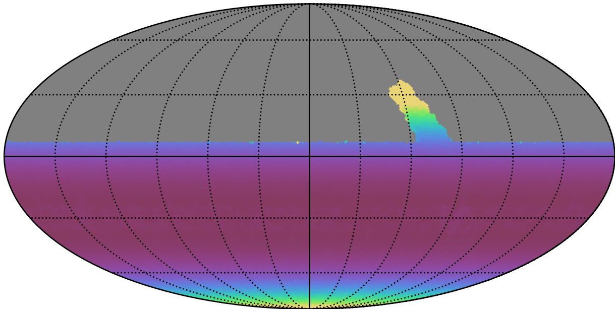
retro_baseline_v2.0_10yrs All sky y band: Min airmass
