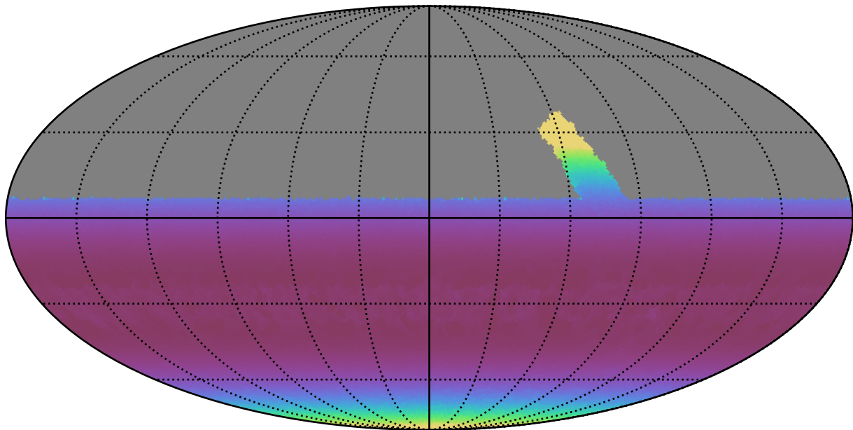
retro_baseline_v2.0_10yrs All sky u band: Min airmass
