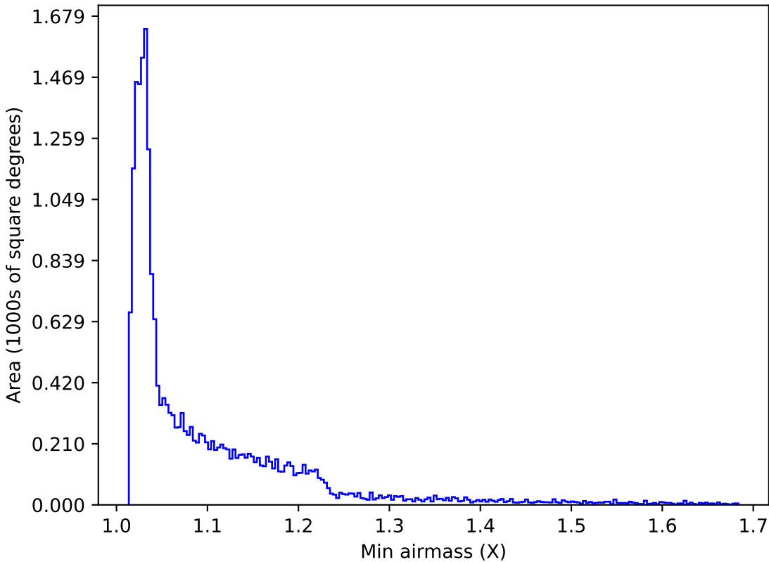
retro_baseline_v2.0_10yrs All sky u band: Min airmass
