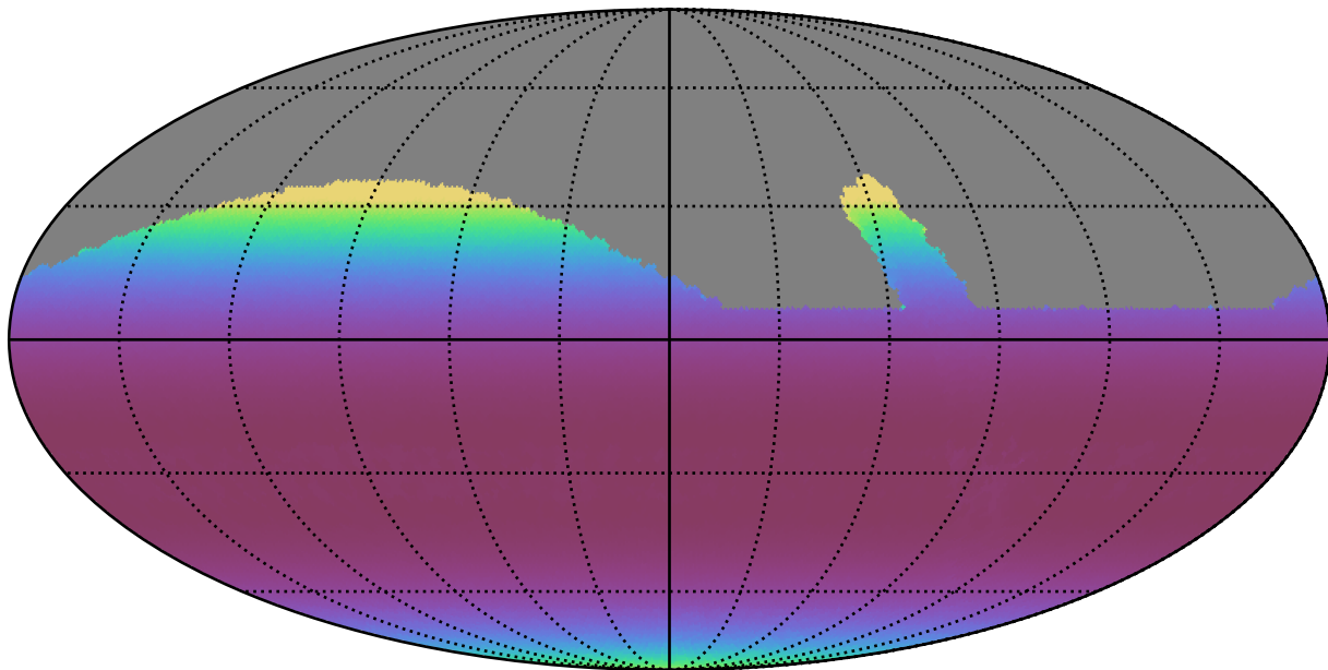
retro_baseline_v2.0_10yrs All sky i band: Min airmass
