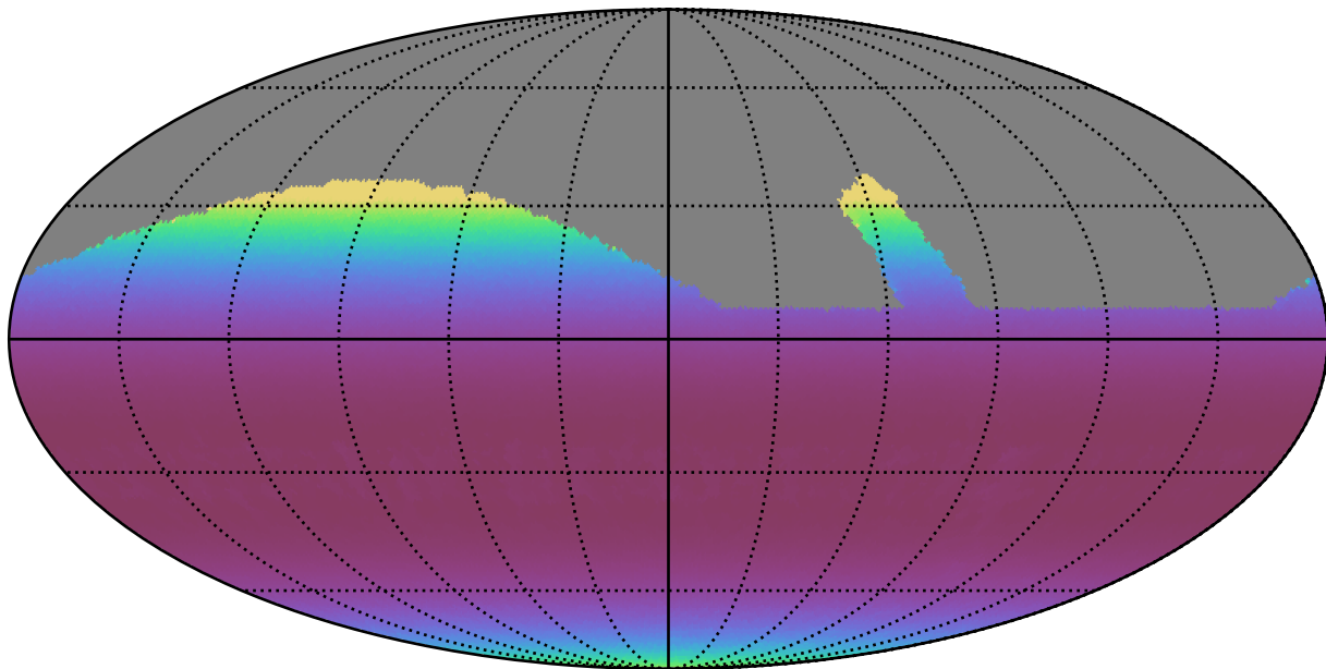
retro_baseline_v2.0_10yrs All sky g band: Min airmass
