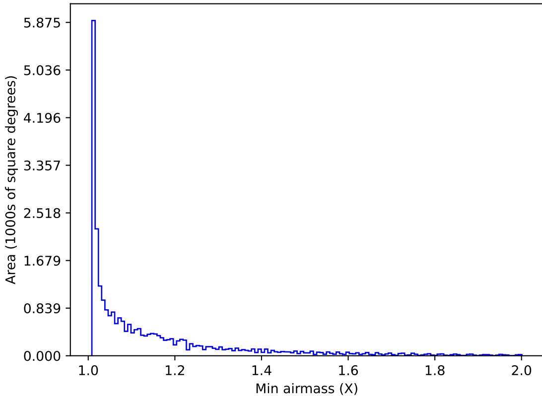
retro_baseline_v2.0_10yrs All sky all bands: Min airmass
