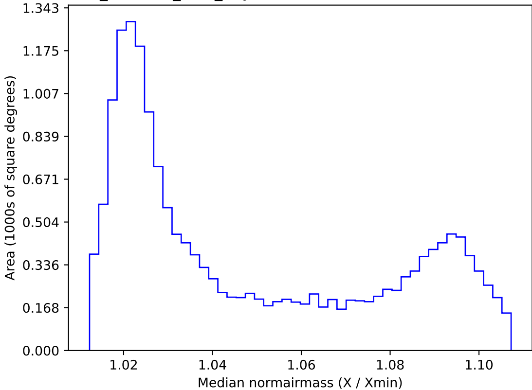
retro_baseline_v2.0_10yrs WFD z band: Median normairmass
