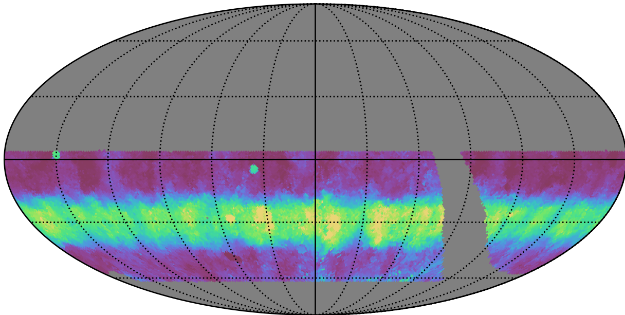
retro_baseline_v2.0_10yrs WFD u band: Median normairmass
