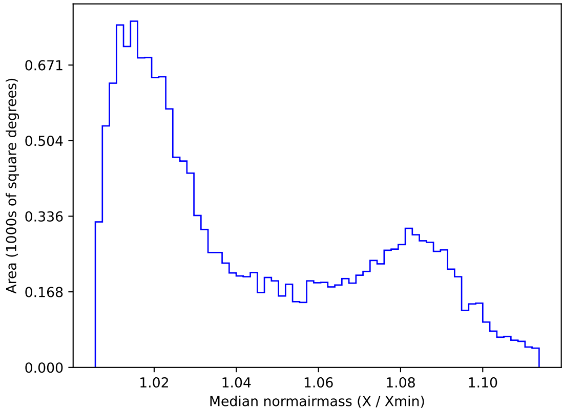
retro_baseline_v2.0_10yrs WFD u band: Median normairmass
