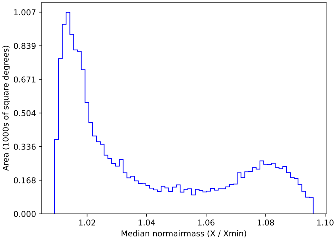
retro_baseline_v2.0_10yrs WFD r band: Median normairmass
