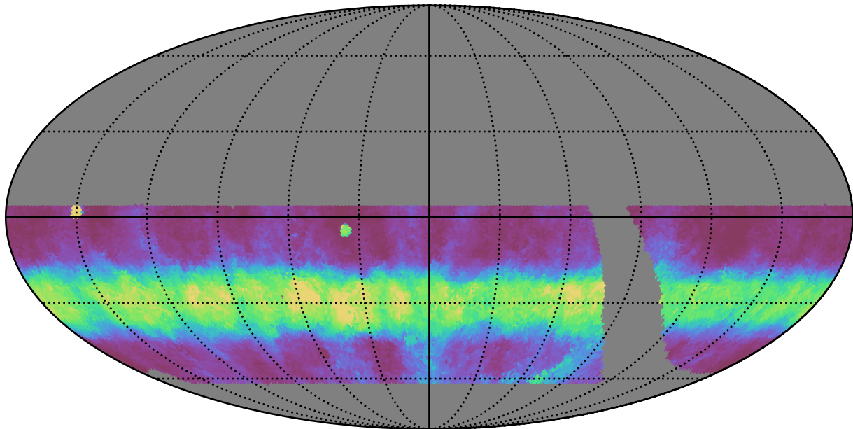
retro_baseline_v2.0_10yrs WFD g band: Median normairmass
