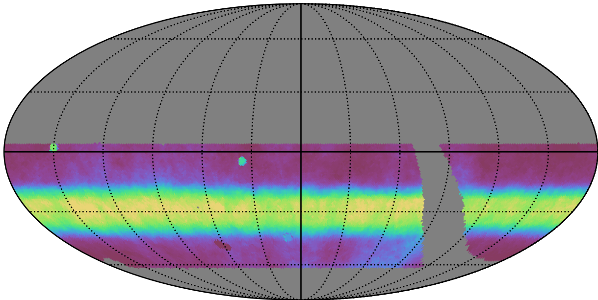
retro_baseline_v2.0_10yrs WFD all bands: Median normairmass
