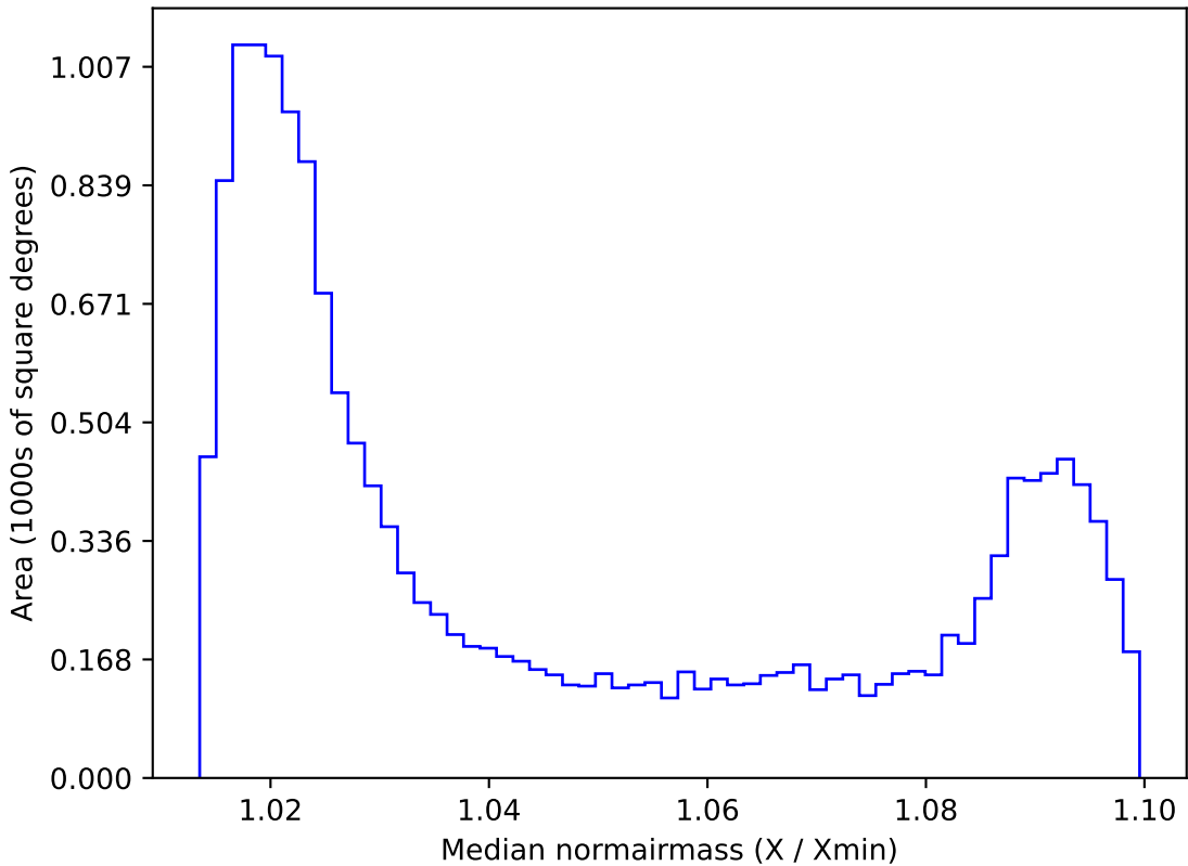
retro_baseline_v2.0_10yrs WFD all bands: Median normairmass
