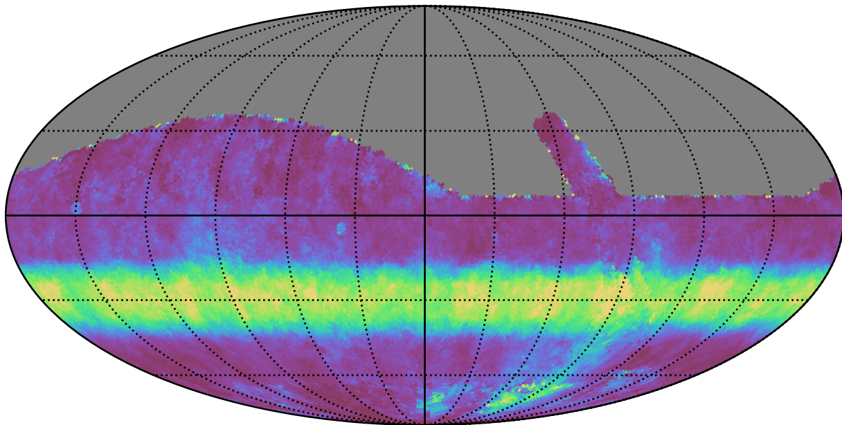
retro_baseline_v2.0_10yrs All sky z band: Median normairmass
