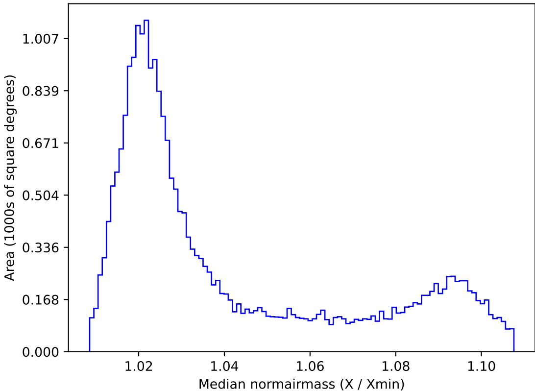
retro_baseline_v2.0_10yrs All sky z band: Median normairmass
