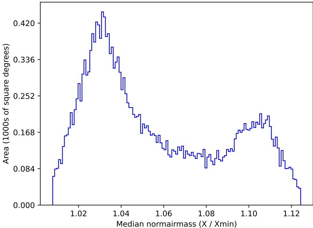
retro_baseline_v2.0_10yrs All sky y band: Median normairmass
