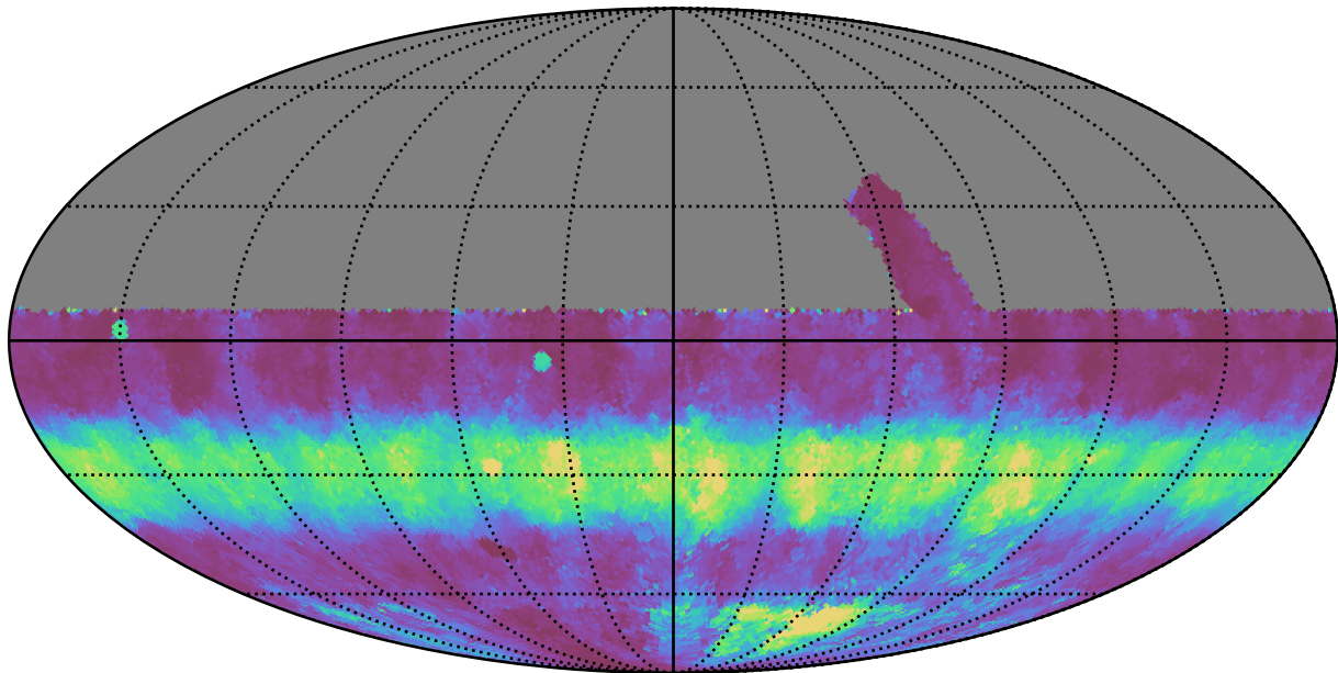
retro_baseline_v2.0_10yrs All sky u band: Median normairmass
