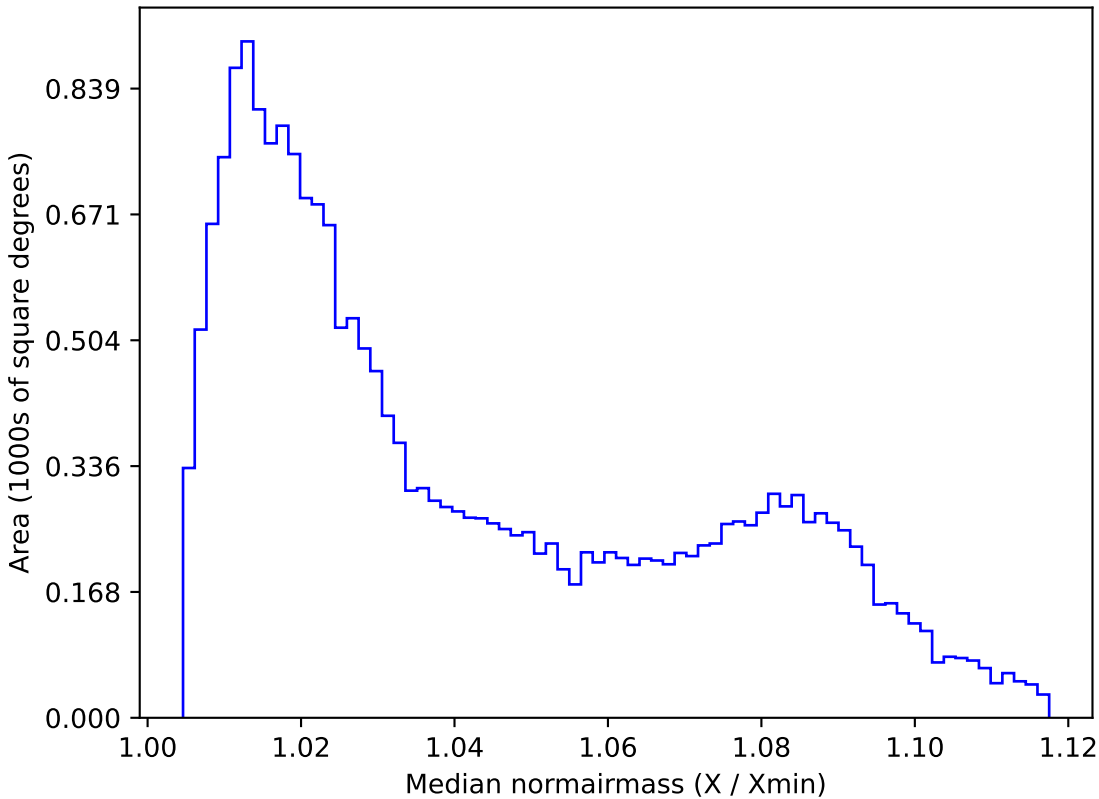
retro_baseline_v2.0_10yrs All sky u band: Median normairmass
