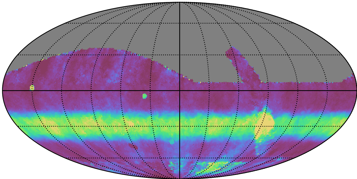
retro_baseline_v2.0_10yrs All sky r band: Median normairmass
