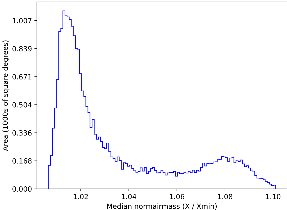
retro_baseline_v2.0_10yrs All sky r band: Median normairmass
