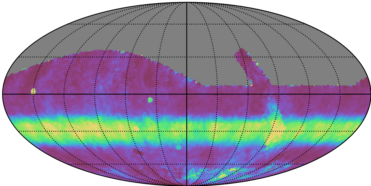
retro_baseline_v2.0_10yrs All sky i band: Median normairmass
