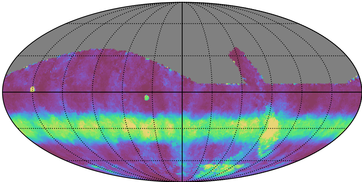
retro_baseline_v2.0_10yrs All sky g band: Median normairmass
