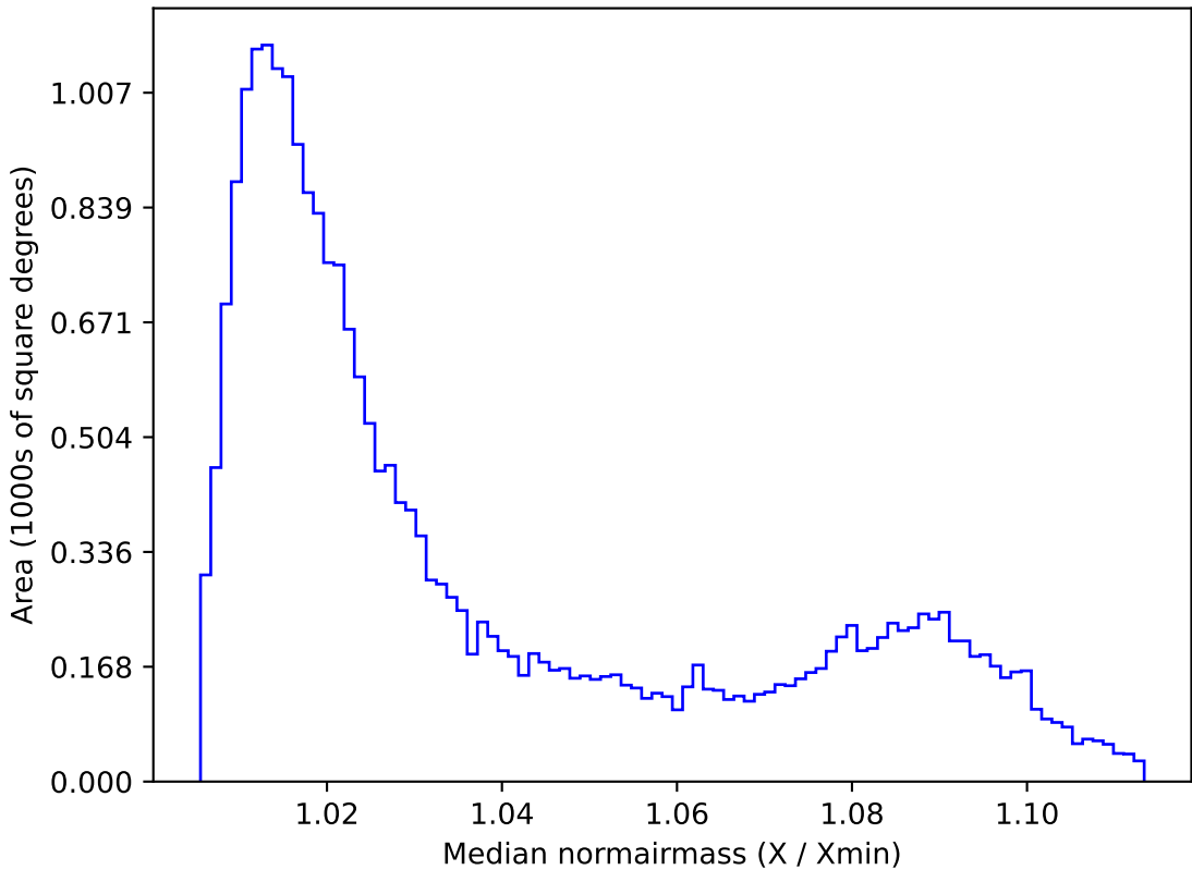
retro_baseline_v2.0_10yrs All sky g band: Median normairmass
