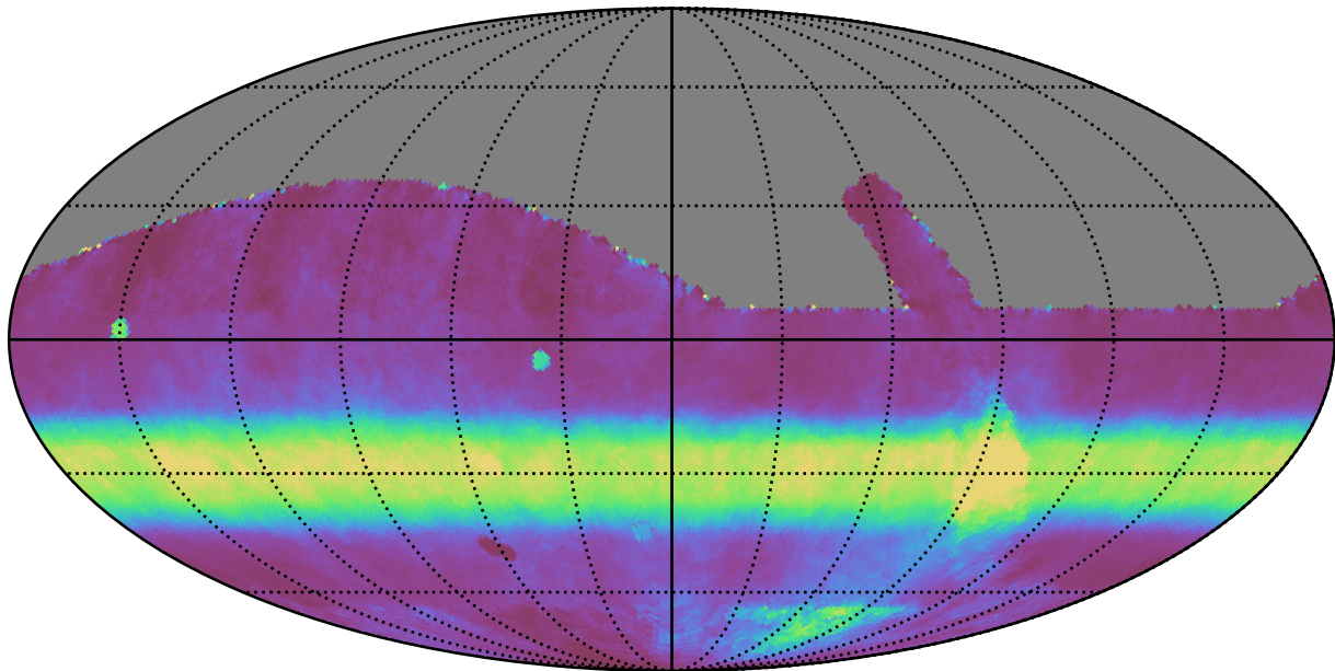
retro_baseline_v2.0_10yrs All sky all bands: Median normairmass
