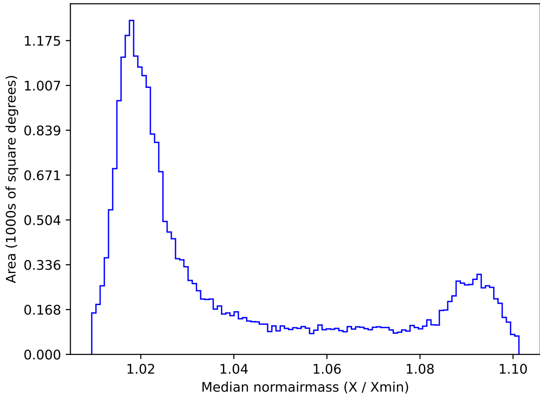
retro_baseline_v2.0_10yrs All sky all bands: Median normairmass
