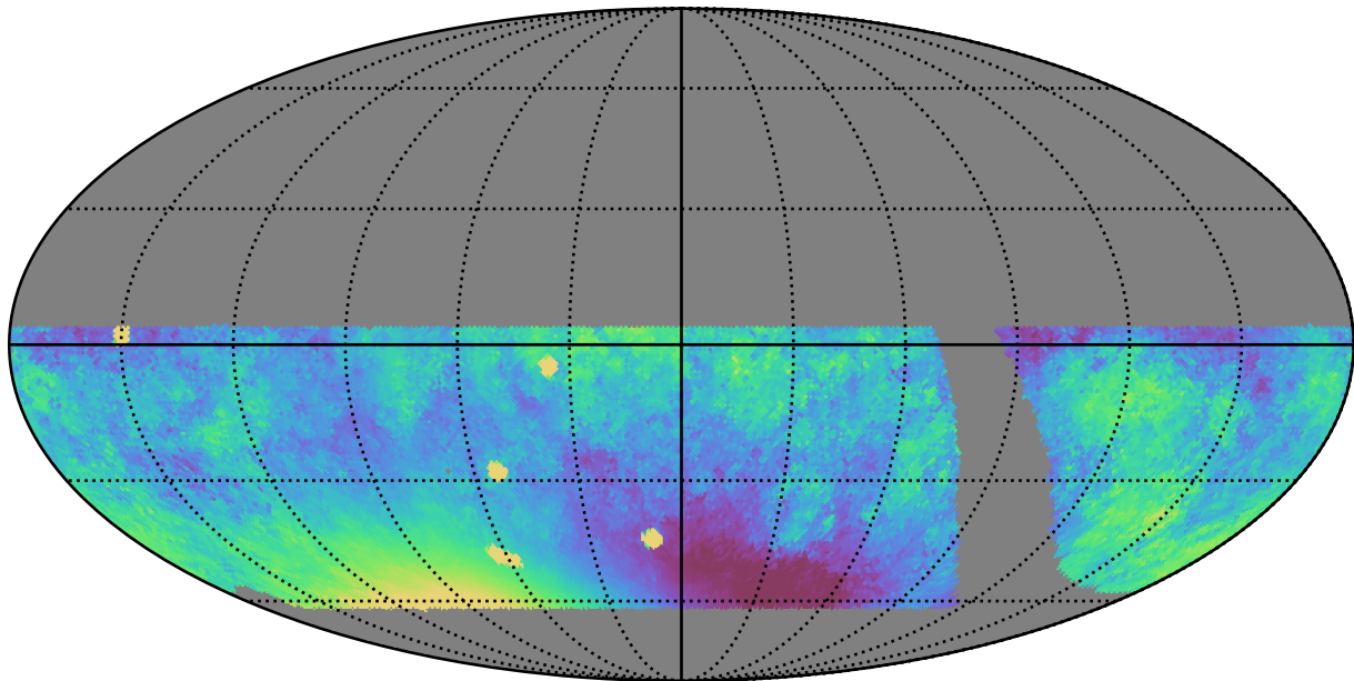
retro_baseline_v2.0_10yrs WFD z band: Median moonDistance
