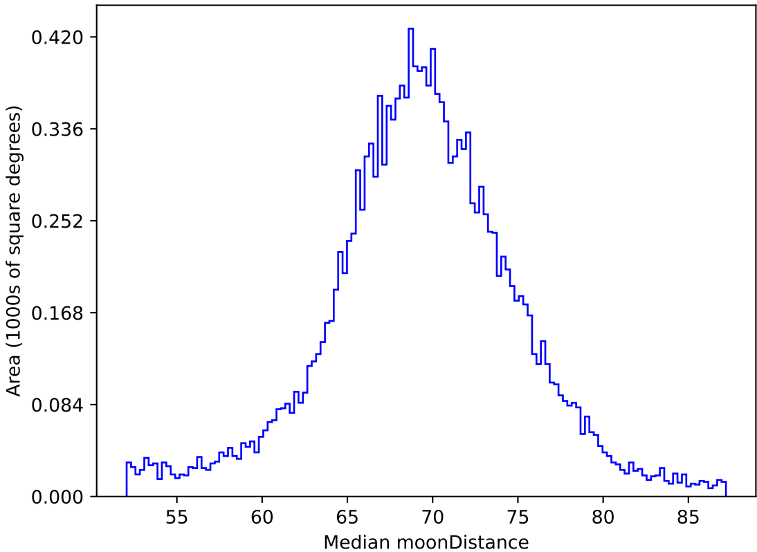
retro_baseline_v2.0_10yrs WFD z band: Median moonDistance
