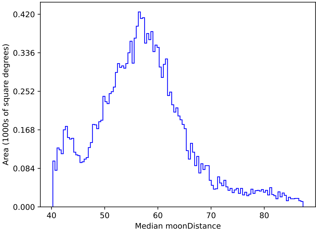
retro_baseline_v2.0_10yrs WFD y band: Median moonDistance
