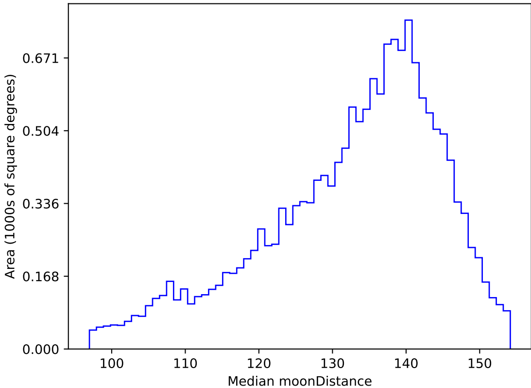
retro_baseline_v2.0_10yrs WFD u band: Median moonDistance
