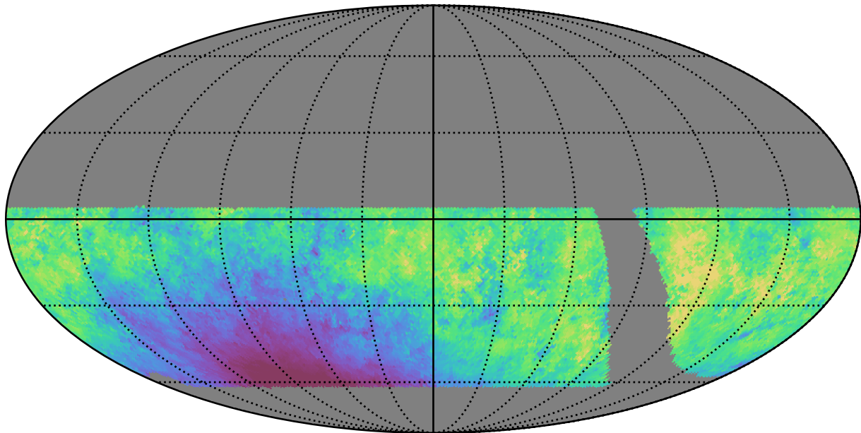
retro_baseline_v2.0_10yrs WFD r band: Median moonDistance
