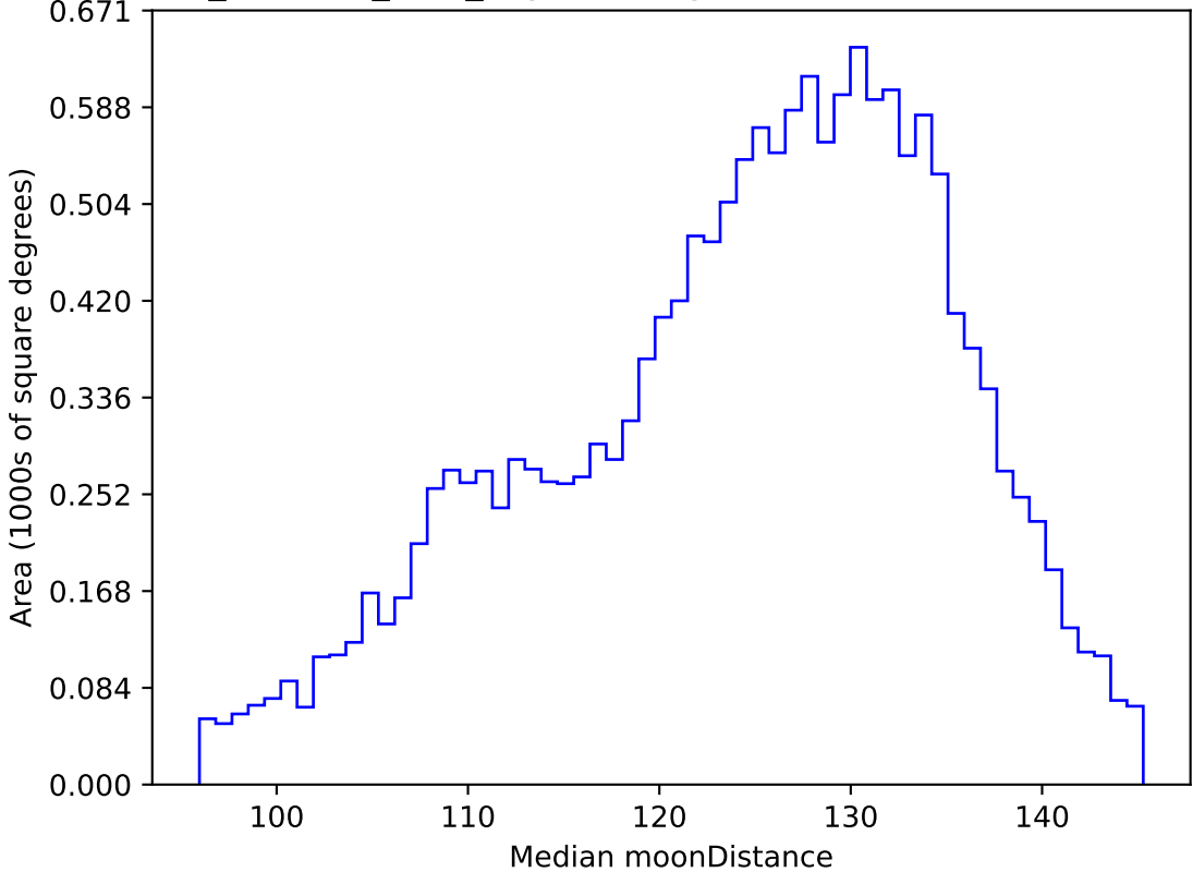
retro_baseline_v2.0_10yrs WFD g band: Median moonDistance
