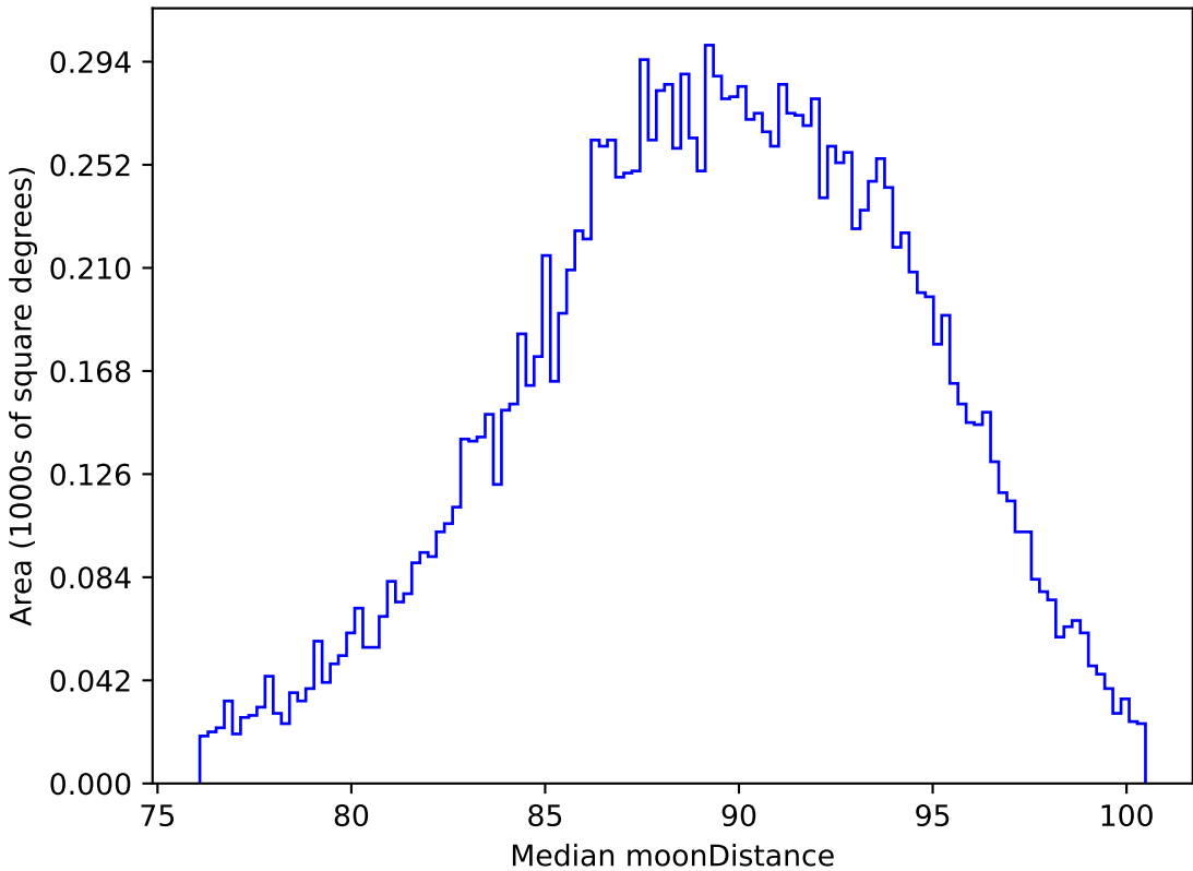
retro_baseline_v2.0_10yrs WFD all bands: Median moonDistance
