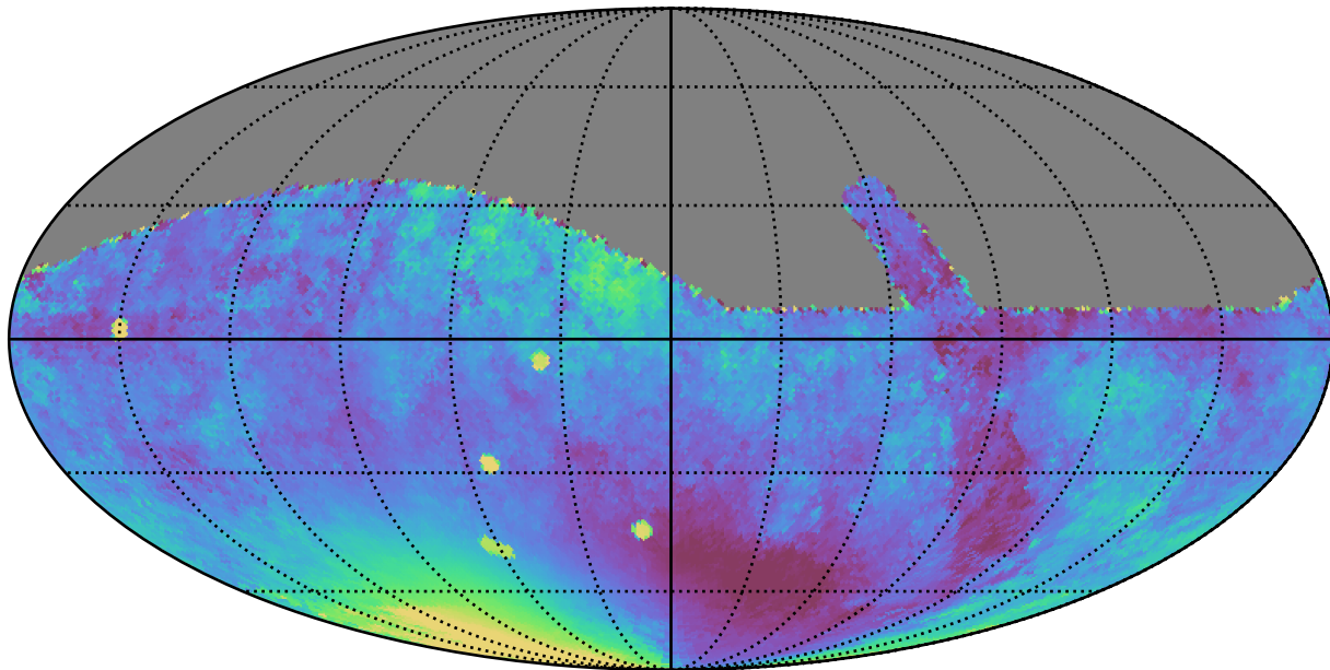
retro_baseline_v2.0_10yrs All sky z band: Median moonDistance
