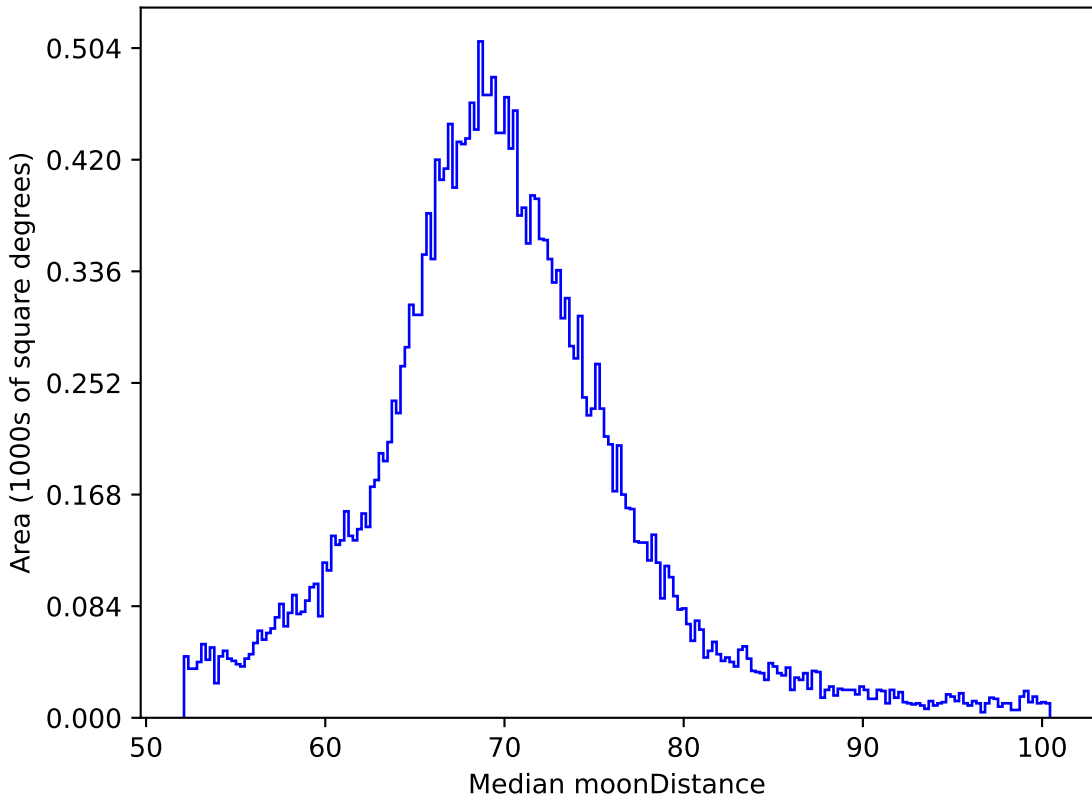
retro_baseline_v2.0_10yrs All sky z band: Median moonDistance
