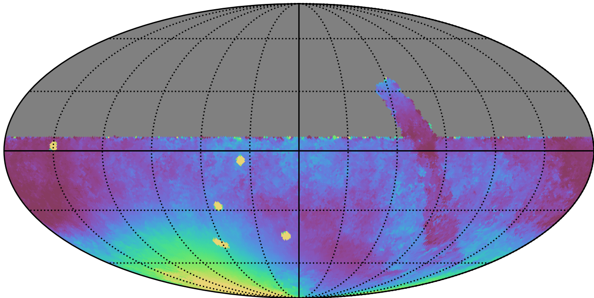
retro_baseline_v2.0_10yrs All sky y band: Median moonDistance
