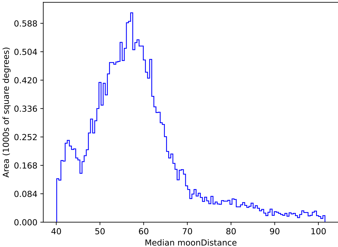
retro_baseline_v2.0_10yrs All sky y band: Median moonDistance
