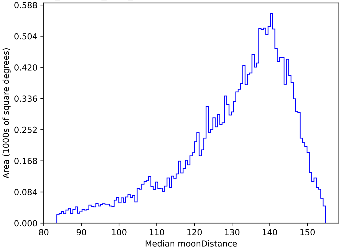
retro_baseline_v2.0_10yrs All sky u band: Median moonDistance
