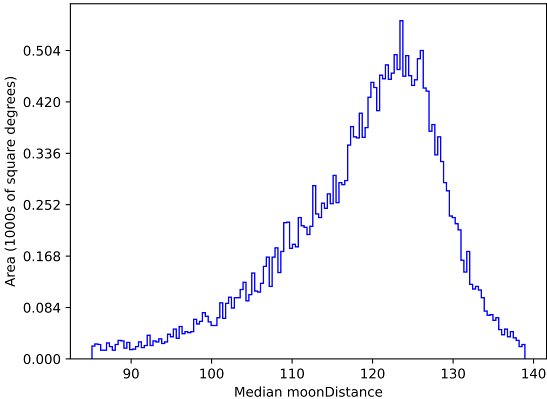
retro_baseline_v2.0_10yrs All sky r band: Median moonDistance
