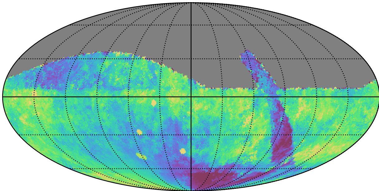
retro_baseline_v2.0_10yrs All sky i band: Median moonDistance
