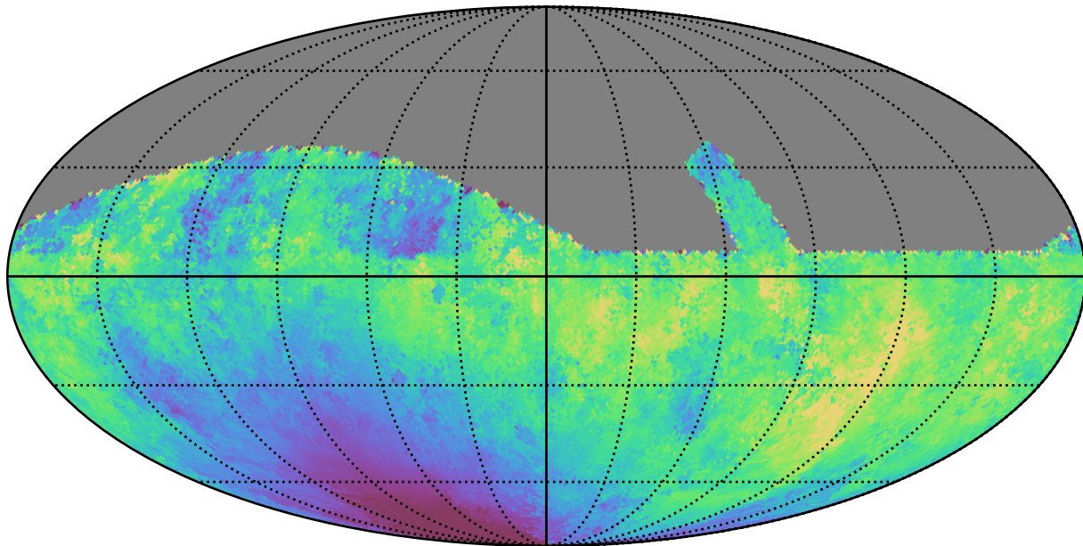
retro_baseline_v2.0_10yrs All sky g band: Median moonDistance
