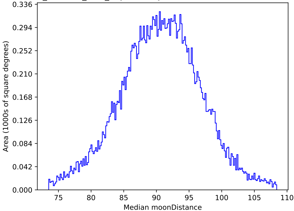
retro_baseline_v2.0_10yrs All sky all bands: Median moonDistance
