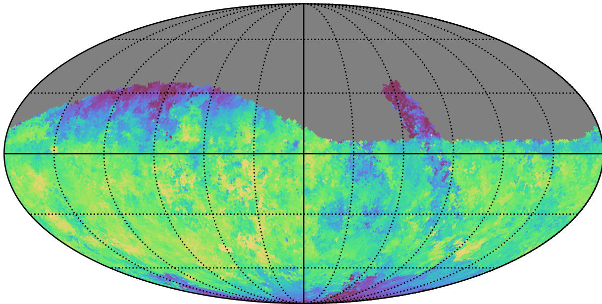
retro_baseline_v2.0_10yrs Yr 1 z band: Median fiveSigmaDepth
