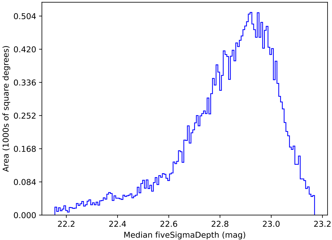
retro_baseline_v2.0_10yrs Yr 1 z band: Median fiveSigmaDepth
