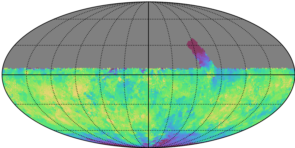
retro_baseline_v2.0_10yrs Yr 1 y band: Median fiveSigmaDepth
