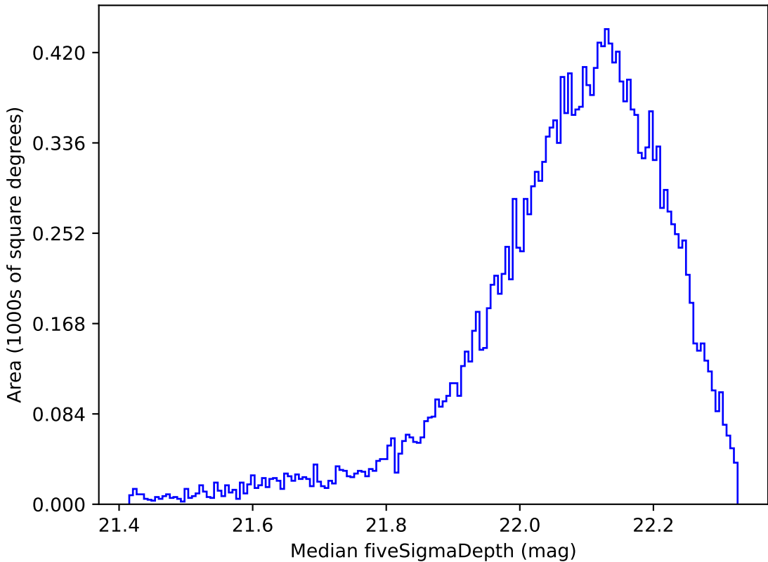
retro_baseline_v2.0_10yrs Yr 1 y band: Median fiveSigmaDepth
